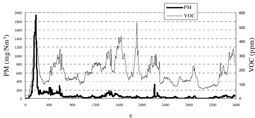
Figure 3. Variation of PM, VOC emission vs time [s] after initial kindling for a closed fireplace filled with beech wood.
