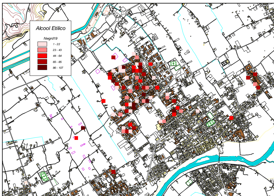
Figure 4 Chromatic map of Ethyl Alcohol emissions [kg/day] in Santa Croce sull'Arno
