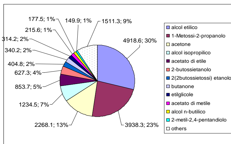
Figura 3a Water Soluble Organic Compound in each plot the quantities are expressed in [kg/day] ; [wt%].
