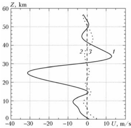
Fig. 3. Monthly average wind velocity components for the equator according to the UARS-UKMO data for October, 2005: zonal (1), meridional (2), and vertical (3) wind component.
