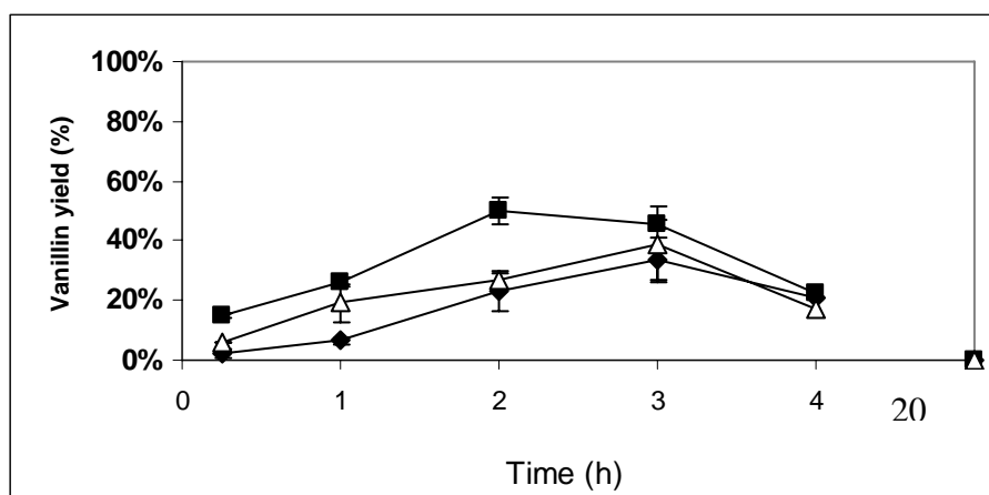
Fig.1: Vanillin molar yields obtained using the undiluted hydrolizate(◆), the hydrolizate diluted 3:1(■), and diluted 1:1 (△)
