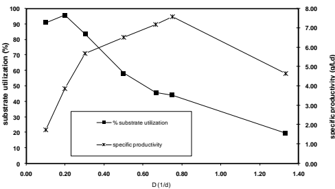
Fig. 5 Substrate utilization and Specific productivity for a single CSTR reactor
