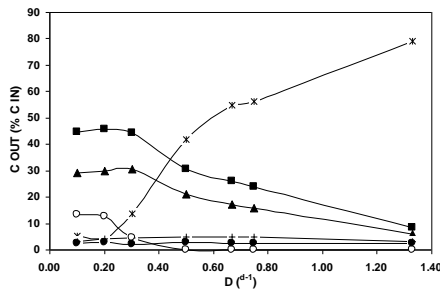
Fig. 2 Carbon mass balance for the single CSTR system
