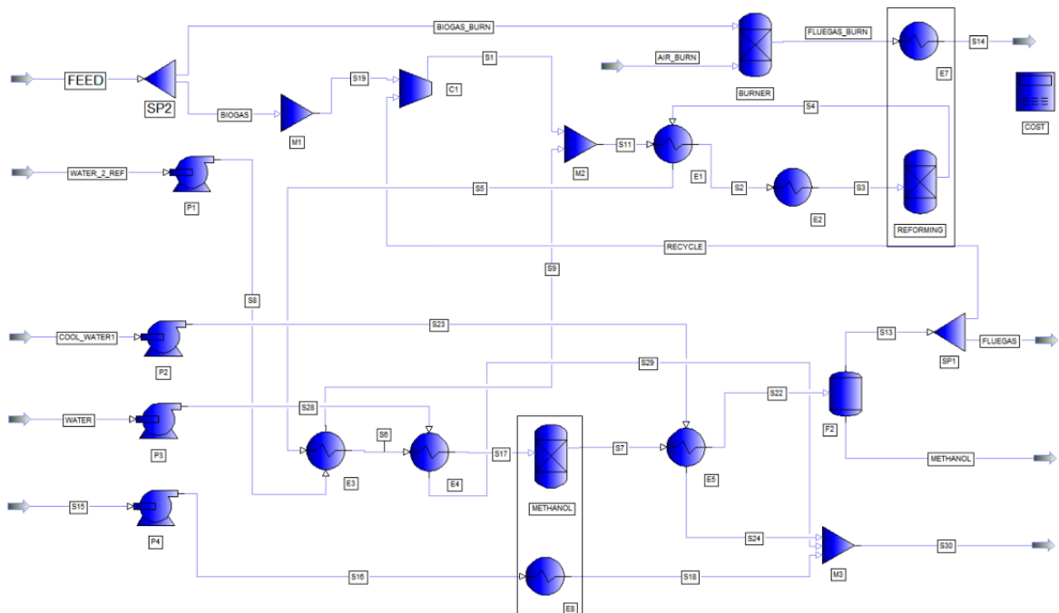
Figure 1: Biogas-to-Methanol process layout.
