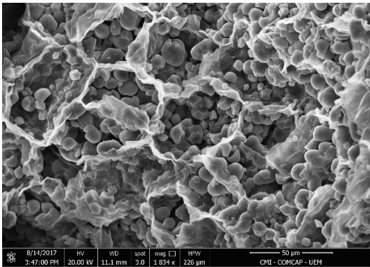
Figure 1: Scanning Electron Microscopy (SEM) analysis of CBR.
