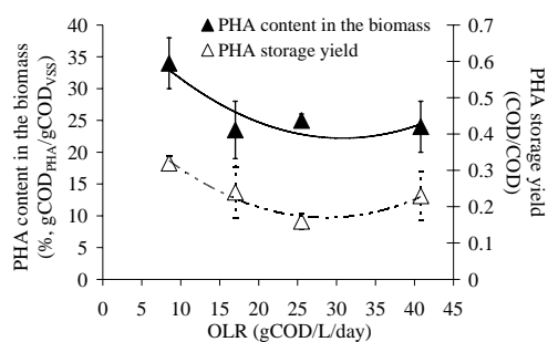
Figure 2. Maximal PHA content in the biomass and the corresponding storage yield, measured in batch accumulation tests.
