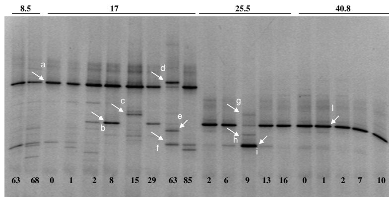
Figure 3. DGGE profiles of SBR runs maintained at increasing OLR values: 8.5, 17, 25.5 and 40.8 gCOD/L/day. Numbers at the bottom of each lane indicate the sampling time in days relative to each run. Arrows and letters indicate bands that have been excised, cloned and sequenced.
