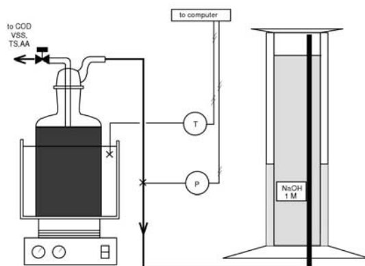
Figure 1. Batch reactor scheme.
