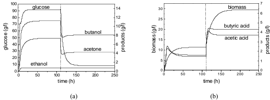
Fig. 2. Simulation results of glucose and products (a), and biomass and the intermediates (b). The vertical dashed line indicates the time when the flash tank separation system is turned on.
