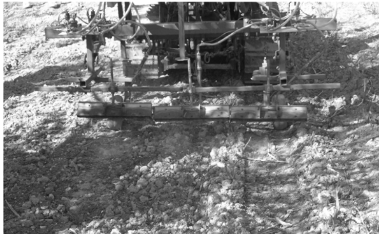
Figure 2: Flaming machine during a post-emergence treatment in garlic
