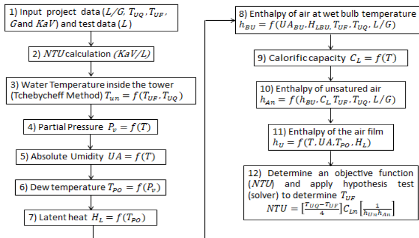
Figure 2: Procedure for determining the water flow temperature at the outlet
