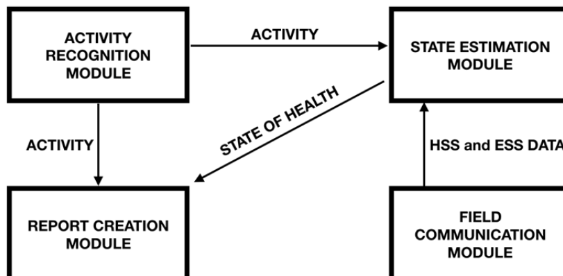
Figure 1: Mobile application logic scheme
