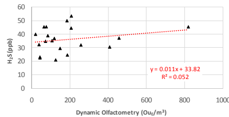
Figure 7: Absence of correlation between H 2 S continuous measurements by Jerome J605 analyzer and ou E /m 3 values obtained by dynamic olfactometry
