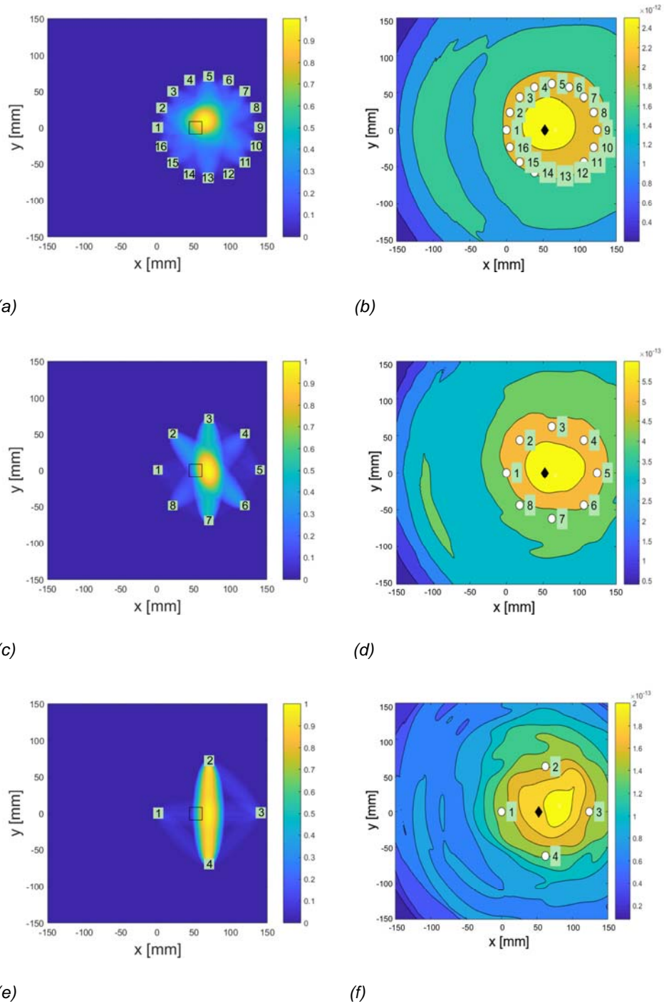
Figure 2: Results for tomography with 16 (a) 8 (c) and 4 (e) sensor and for wave scattering with 16 (b) 8 (d) and 4 (f) sensors. Notch at (52.49, 0) mm and depth of 3 mm. Empty square denotes notch size and position whilst black diamonds only position.
