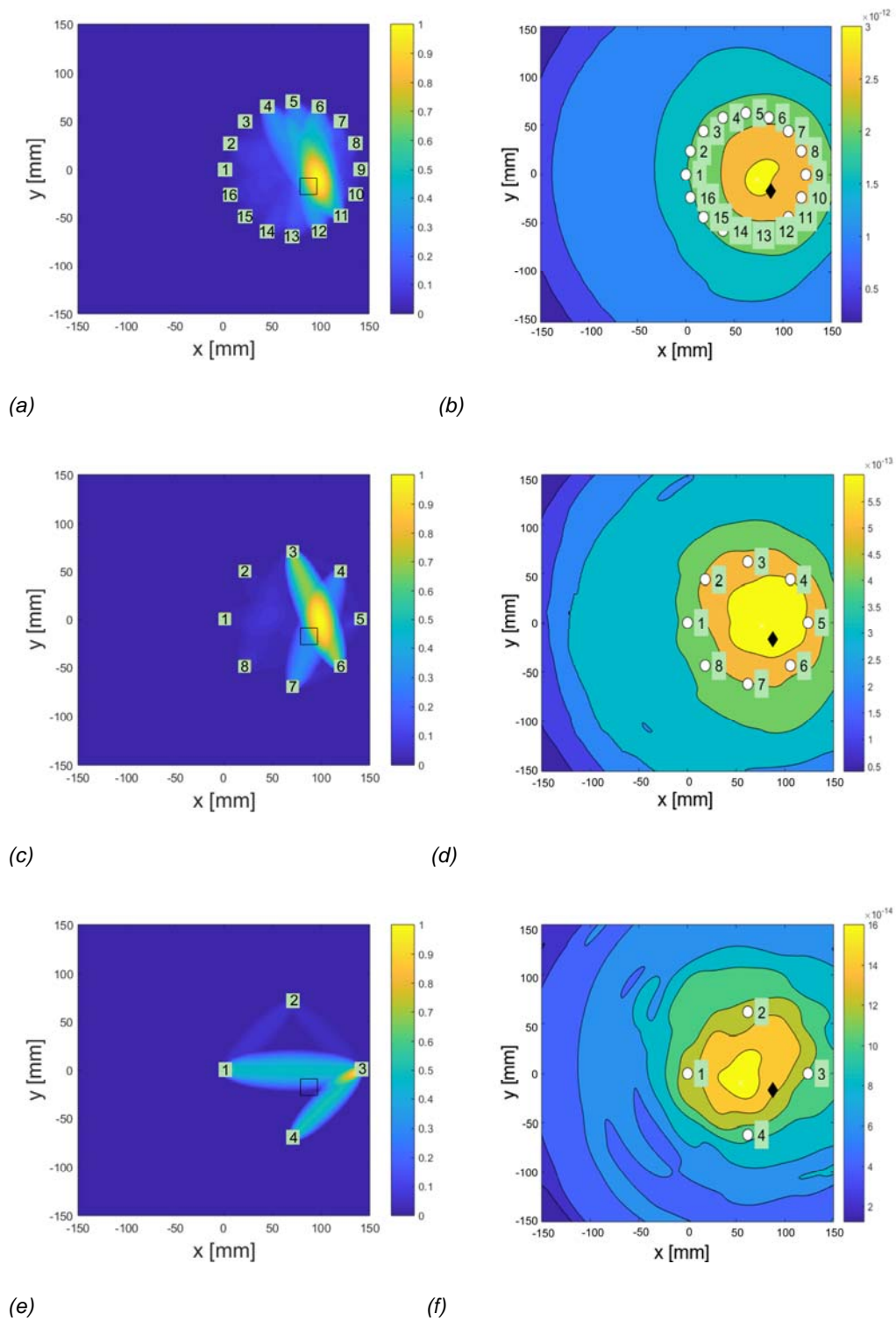
Figure 3: Results for tomography with 16 (a) 8 (c) and 4 (e) sensor and for wave scattering with 16 (b) 8 (d) and 4 (f) sensors. Notch at (87.48, -17.50) mm and depth of 3 mm. Empty square denotes notch size and position whilst black diamonds only position.
