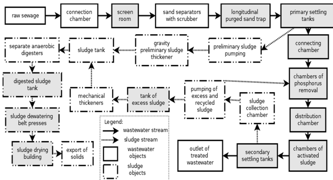
Figure 1: Technological scheme of Wastewater Treatment Plant
