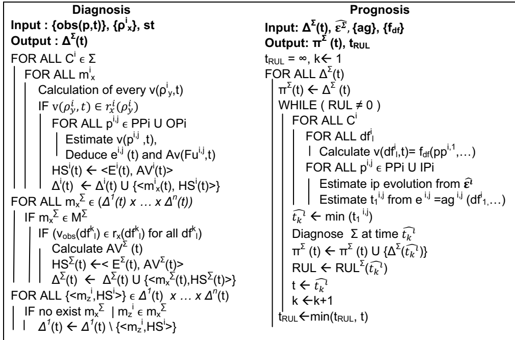
Figure 3: Diagnosis and prognosis algorithms
