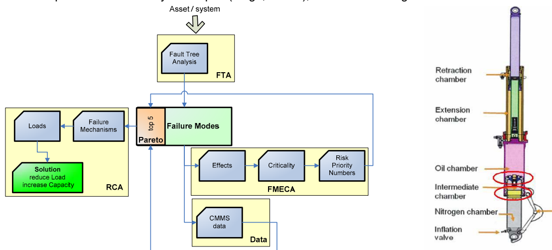
Figure 2: Mechanism based Failure Analysis: selection of the most critical components and the associated failure mechanism and loads.
