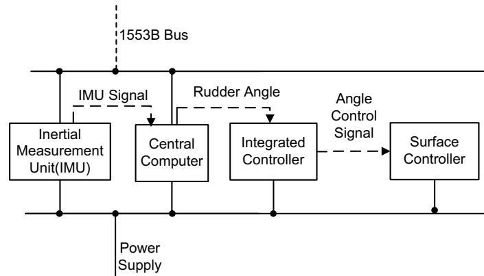
Figure 3: Structure of flying control system
