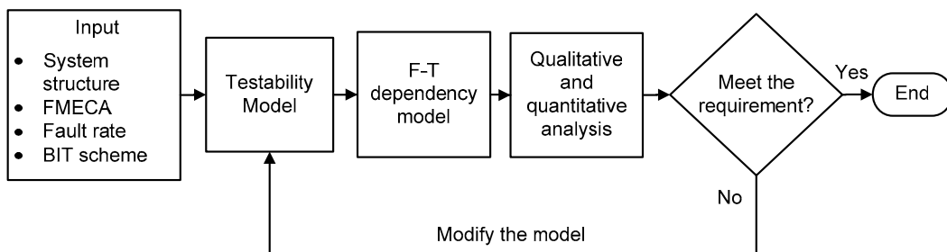
Figure 1: Iterative process of analysis and modification in testability design
