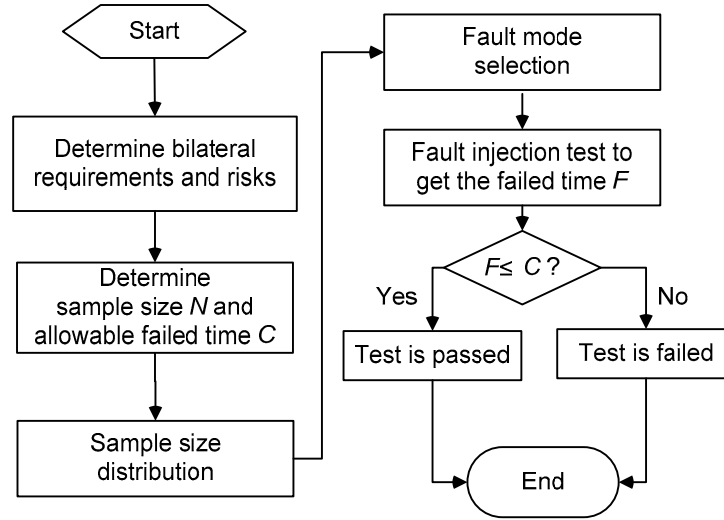
Figure 2: Flow chart of the physical test demonstration
