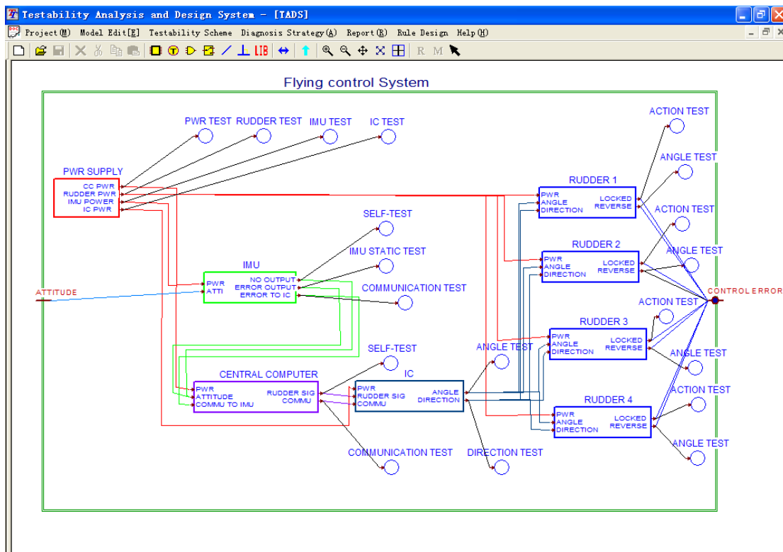
Figure 4: Testability model of flying control system with TADS
