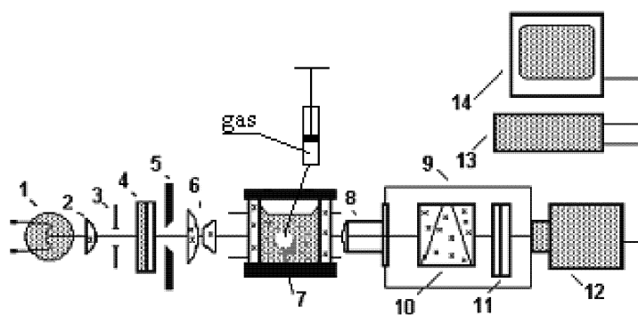
Fig. 1. Polarizing interference microscope: (1) filament lamp; (2) lens; (3) aperture; (4) polarizer; (5) slit-shaped aperture; (6) condenser; (7) cell; (8) microlens; (9) polarizing interference unit; (10) prism; (11) analyzer; (12) TV camera; (13) video type recorder, and (14) TV monitor
