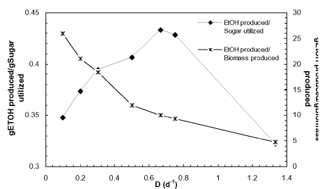
Fig. 4 EtOH produced/Sugars utilized and EtOH produced/Biomass produced for a single CSTR reactor
