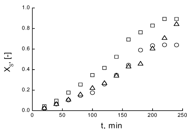
Figure 1. Substrate conversion as a function of process time. [\text{S}]_0 (mM): \square , 20; \triangle , 40; \circ , 60.
