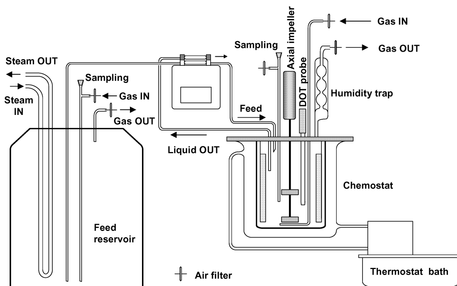
Figure 1 – Experimental apparatus.
