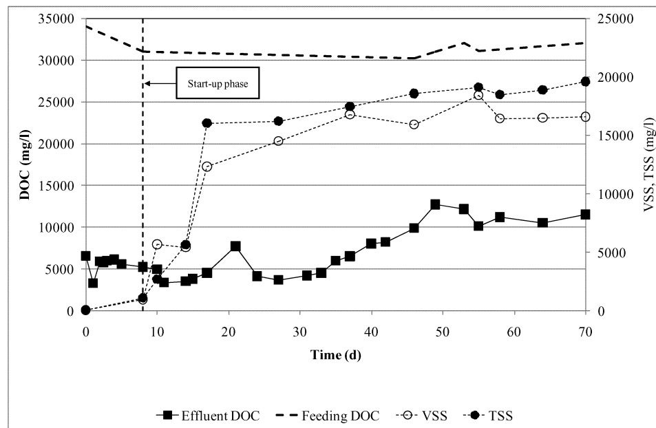
Figure 2 – Biomass profile and COD concentration in the outcoming effluent.
