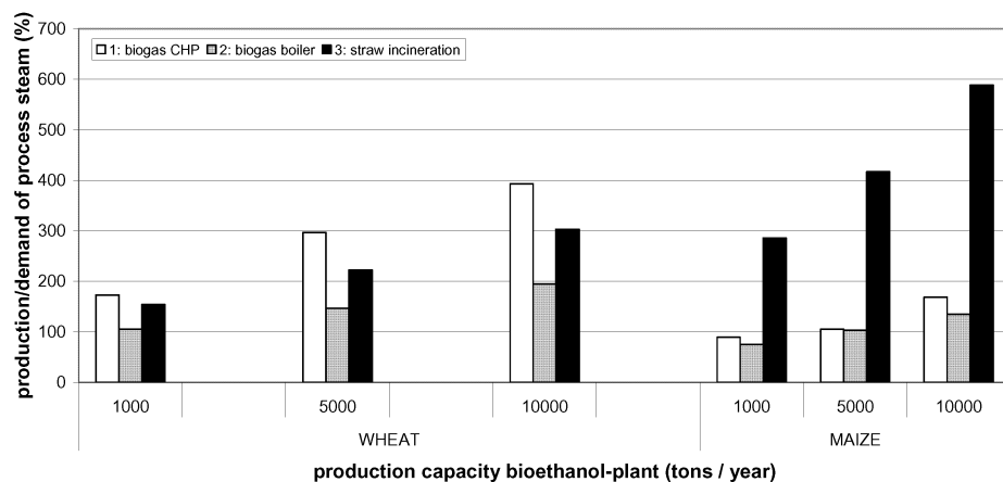
Figure 2: Coverage of energy demand of the bioethanol production from wheat and maize for 3 different production capacities
