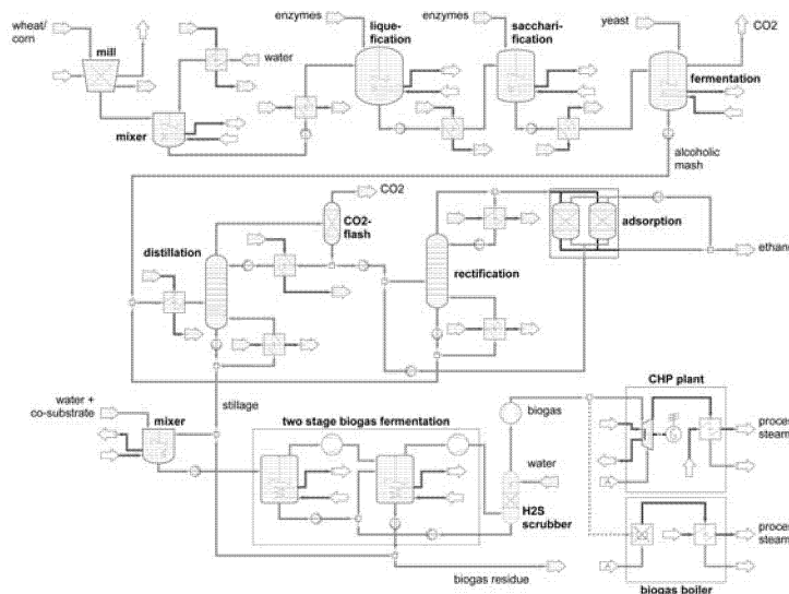
Figure 1: IPSEpro simulation model of coupled bioethanol and biogas production; biogas utilisation in CHP and biogas boiler, respectively
